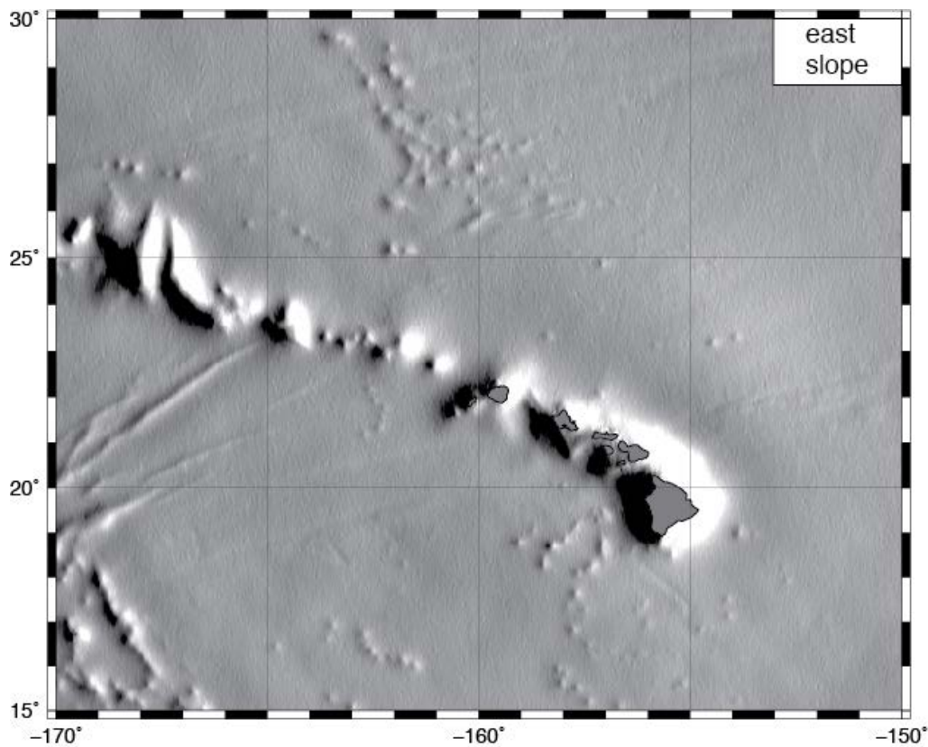
Figure 5. East component of sea surface slope \eta(x) derived from Geosat and ERS altimeter profiles. Note this component is rather noisy because the altimeter tracks (Figure 3) run mainly in a N-S direction.
