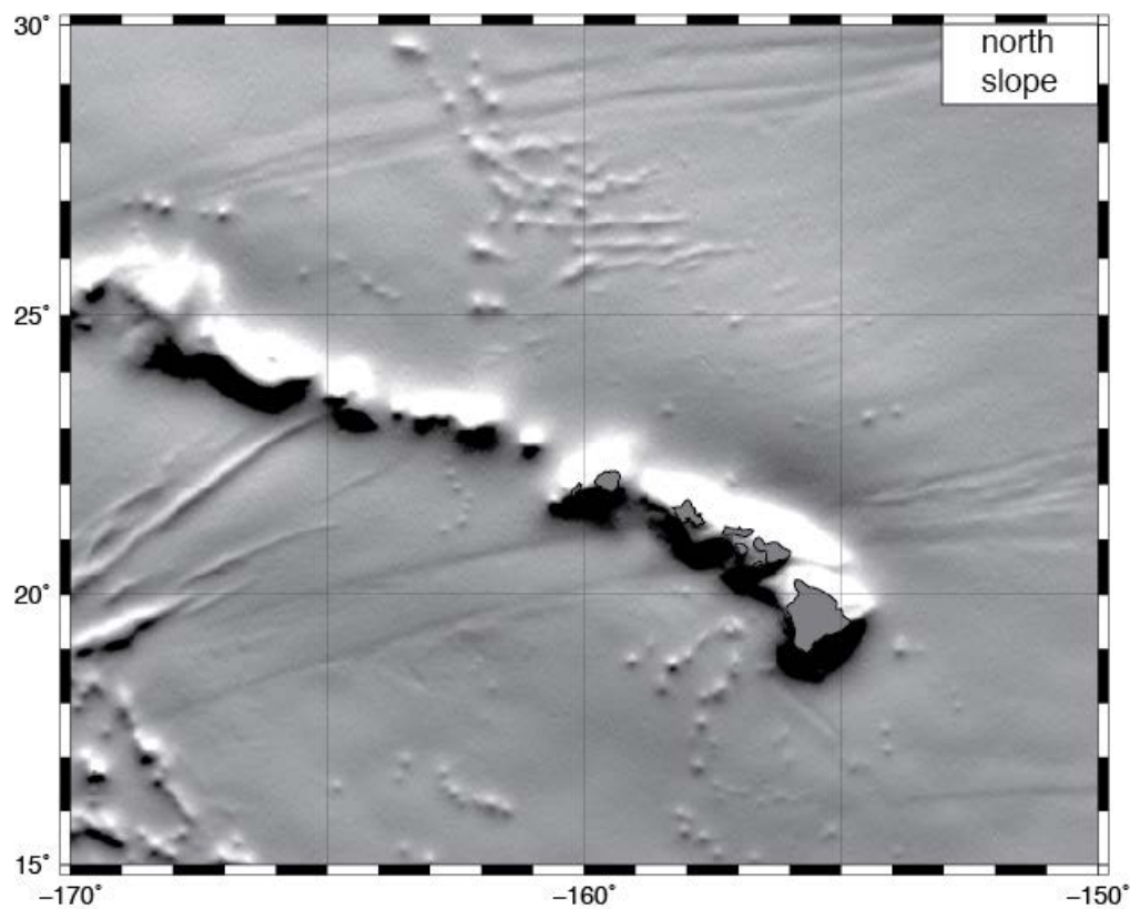
Figure 6. North component of sea surface slope \xi(x) derived from Geosat and ERS altimeter profiles. Note this component has lower noise because the altimeter tracks (Figure 3) run mainly in a N-S direction.
