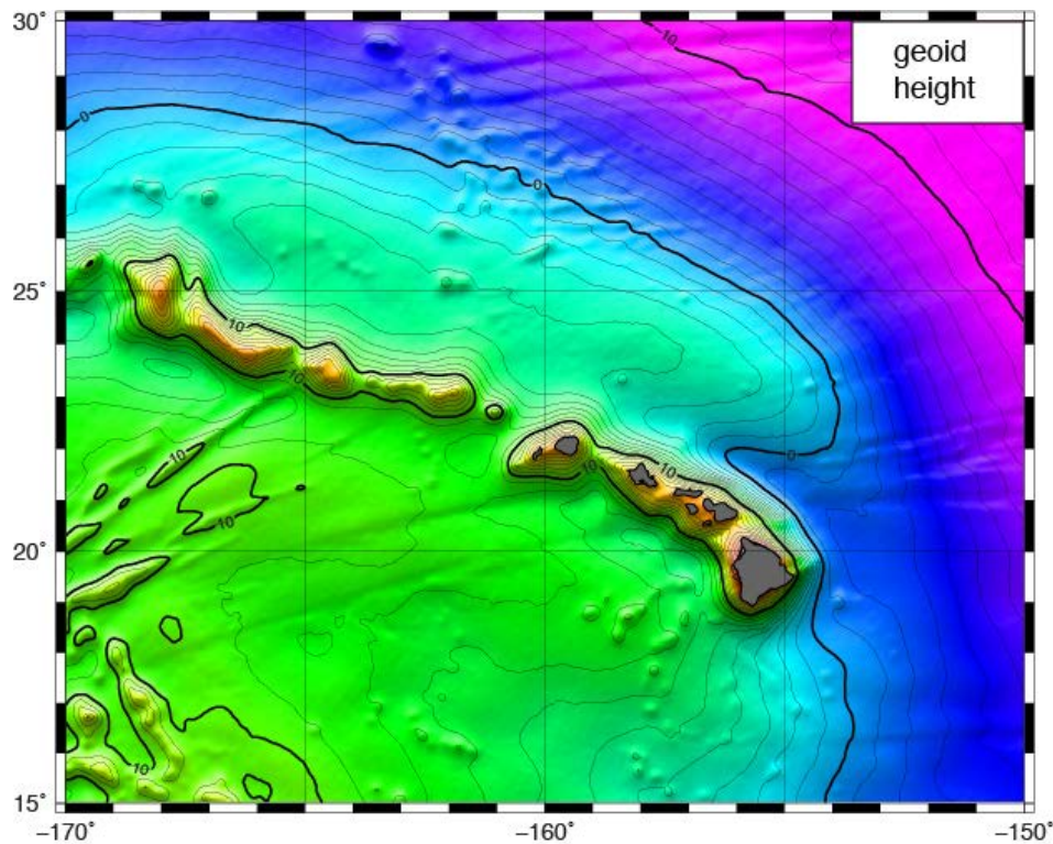
Figure 4. Geoid height above the WGS84 ellipsoid in meters (1-m contour interval) from EGM2008 [Pavlis et al. , 2008]. The geoid height is dominated by long-wavelengths so it is difficult to observe the small-scale features caused by ocean-floor topography. These can be enhanced by computing either the horizontal derivative (ocean surface slope) or the vertical derivative ( gravity anomaly).
