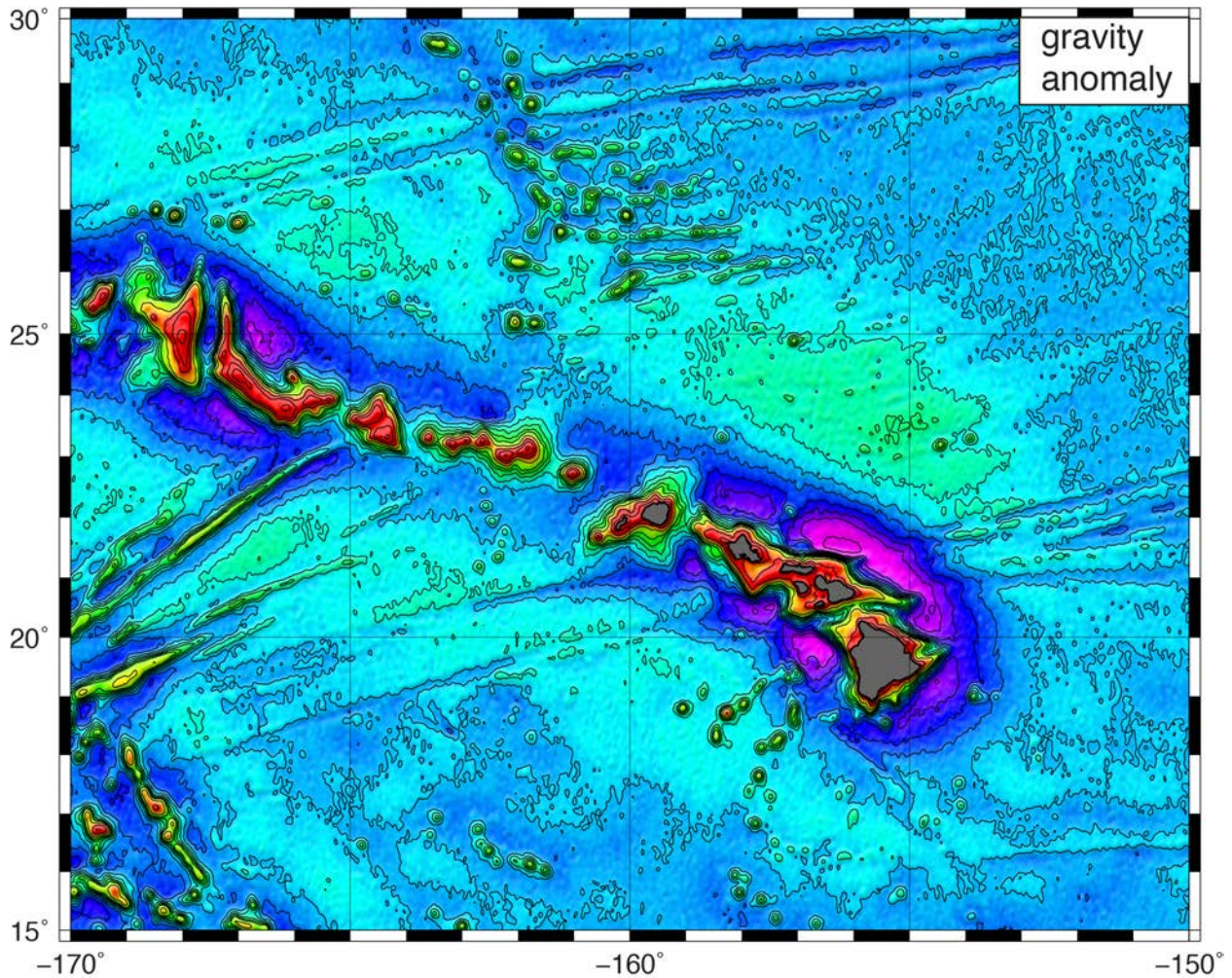
Figure 7. Gravity anomaly \Delta g(\mathbf{x}) derived from east and north components of sea surface slope using equation (14). (20 mGal contour interval)
