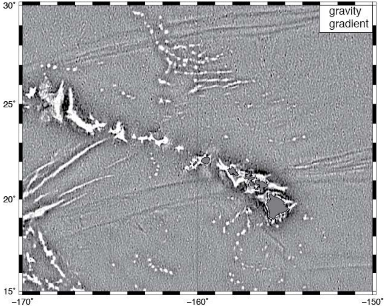
Figure 8. Vertical gravity gradient \partial g(\mathbf{x})/\partial z derived from east and north components of sea surface slope using equation (15). Note this second derivative of the geoid amplifies the shortest wavelengths; compare with the original geoid (Figure 3). Noise in the altimeter measurements has been amplified resulting in an artificial texture.
