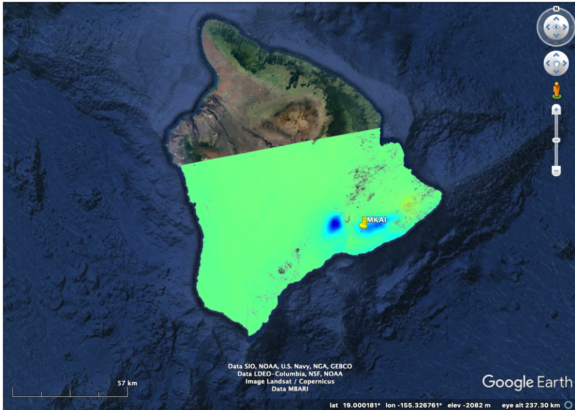
Location of GNSS station MKAI, near Kilauea.
