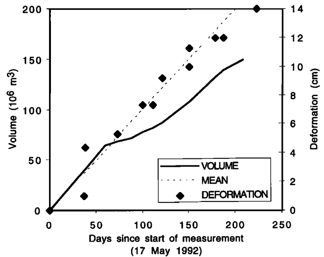
Figure 11. Subsidence of the summit of Etna as a function of time [ Massonnet et al. , 1995a]. The values are deduced from the models that best fit the observed interferograms. The result shows a linear relation between time and displacement that implies a constant rate of volume loss for the volcano (dashed line). The solid line shows the lava production as inferred from field measurements [ Smithsonian Institution , 1991–1993].
