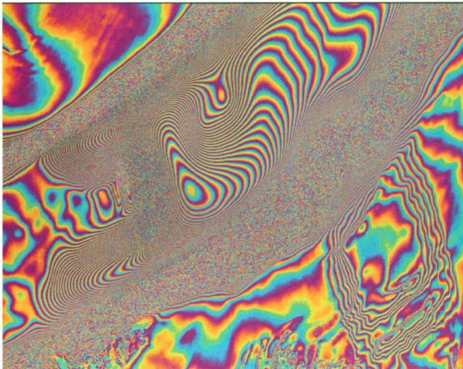
Plate 26. (left) Interferogram showing glacier ice flowing at \sim 1 \text{ m d}^{-1} in Rutford Ice Stream, Antarctica, from Goldstein et al. [1993]. The center of the image is at 78^{\circ}43'S, 83^{\circ}0'W . The radar line-of-sight azimuth ( 350.8^{\circ}T ) is up. Each cycle of color represents 28 mm of range change. (right) Location map for features in the interferogram at left. Ice flow is indicated schematically by arrows. The grounding line is shown dotted. (right from this line, the ice is grounded; downstream, it is afloat. Dash-dot lines show flow traces, faintly visible in the interferogram. The accelerating zone appears as dense fringes south of "bright patch." Goldstein et al. attribute the high velocities to the ocean tides acting on the floating ice. The fringe count indicates that about 2 m of vertical displacements occurred in the 6 days between the two radar images, assuming that the horizontal contribution is given by the ground-based velocity measurements. A tidal rise of 2.1 \pm 0.2 \text{ m} is calculated from empirical Fourier components of the tide observed near Rutford Ice Stream. The shape of the tidal uplift profile measured by the interferogram indicates that the ice shelf flexes upward as it floats. A model describing the flexure as a bending elastic beam provides a good fit to the radar data along the 10 km where the uplift profile is steepest. Reprinted with permission from Goldstein et al. [1993]. Copyright 1993 American Association for the Advancement of Science.
