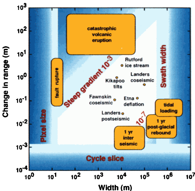
Plate 17. Classification of crustal deformation signals by width and range change. To be detected by interferometry, a signal must fall within the white irregular pentagon. Each of its sides indicates a different physical limit, as described in section 4.1.
