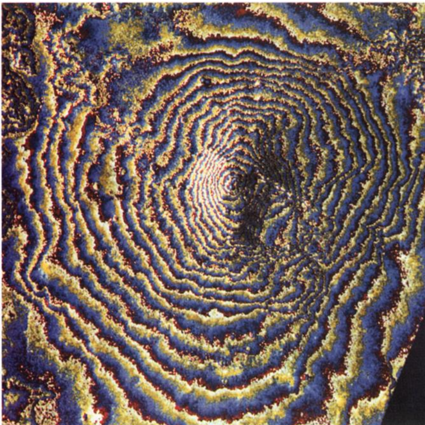
Plate 2. Topographic fringes on Mount Etna. The usual CNES processing has been altered to leave topographic fringes uncorrected while transforming the geometry to map coordinates. Here one fringe represents about 250 m of topographic elevation. The shading represents the topographic relief from the DEM, as if the illumination came from the west. The area is roughly 40 by 40 km.
