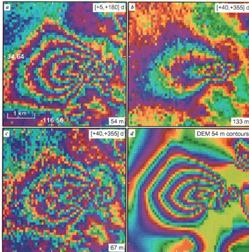
Plate 13. Anomalous rhomboid feature produced by a DEM error in several interferograms near Landers, California [Massonnet and Feigl, 1995a]. (a) Interferogram spanning the interval [+5, +180] d (relative to the Landers mainshock) with altitude of ambiguity h_a = 54 m. One complete cycle of color corresponds to one cycle (28 mm) of change in range. Time intervals are at upper right, h_a is at bottom right, and tick marks are every 0.02^\circ in latitude and longitude. (b) Interferogram spanning the interval [+40, +355] days, with h_a = 133 m. (c) Same interferogram as in Plate 1b, but multiplied by an integer factor of 2 to simulate h_a = 67 m, similar to Plate 13a. (d) Corresponding section of the DEM with a contour interval equal to the 54-m value of h_a for Plate 13a. Plate 13a exhibits a rhomboid feature with four fringes (12 cm) [Massonnet and Feigl, 1995a]. The feature also appears, but as only two fringes, in Plate 13b, where h_a = 133 m. Multiplying the interferogram in Plate 13b by an integer factor of 2 produces Plate 13c, which, with an effective h_a of 66 m, resembles Plate 13a. Therefore the rhomboid feature results from an error of \sim 250 m in the DEM, roughly 8 times larger than the published precision [U.S. Geological Survey (USGS), 1993]. The contoured DEM (Plate 13d) reveals a hill that is not present in the 1:62,500 USGS topographic map [USGS, 1955]. The shape of the fictitious peak in the DEM is reproduced in the interferograms.
