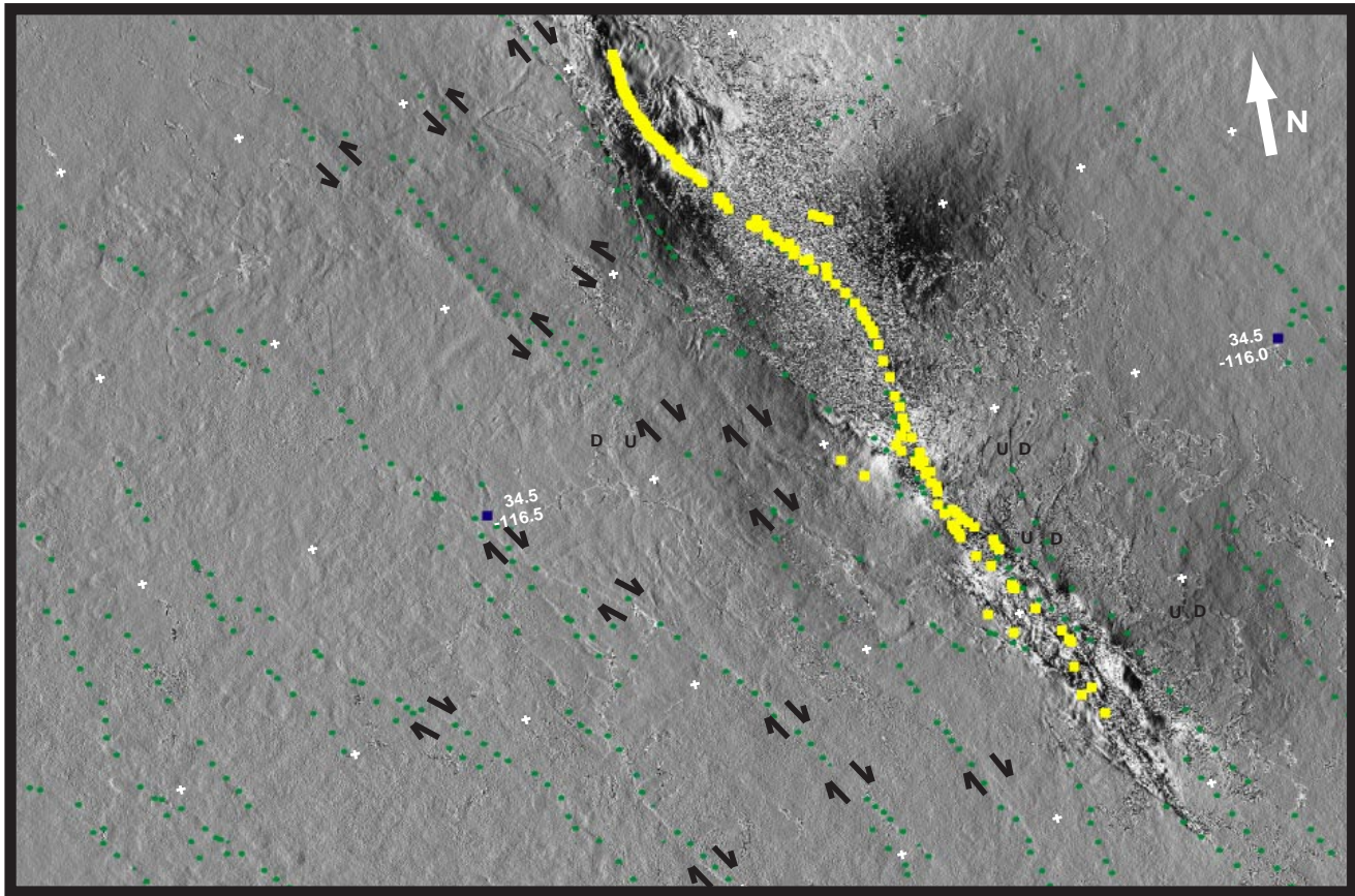
Figure 4. Lineaments in the east component of phase gradient follow previously mapped faults [green dots Jennings 1994 ] and represent small amounts of triggered slip in both right-lateral (or west-side-down) and left-lateral (or west-side-up) directions. Most of the triggered slip lies between the Landers and Hector Mine ruptures. The Emerson fault shows right-lateral triggered slip. Complex zones of surface fracturing and deformation surround the main rupture.
