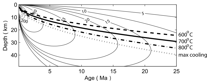
Figure 2. Thin solid curves depict contours of cooling rate ( ^{\circ}\text{C Ma}^{-1} ) as a function of depth and age. Contours converge at zero depth in the youngest part of the lithosphere. Dashed curve, bold solid curve, and dash-dotted curve, respectively, show the 600^{\circ}\text{C} , 700^{\circ}\text{C} , and 800^{\circ}\text{C} isotherm. Dotted curve represents the locus of fastest cooling, which corresponds to an isotherm of 888^{\circ}\text{C} . After Bratt et al. [1985] and Wessel [1992].
