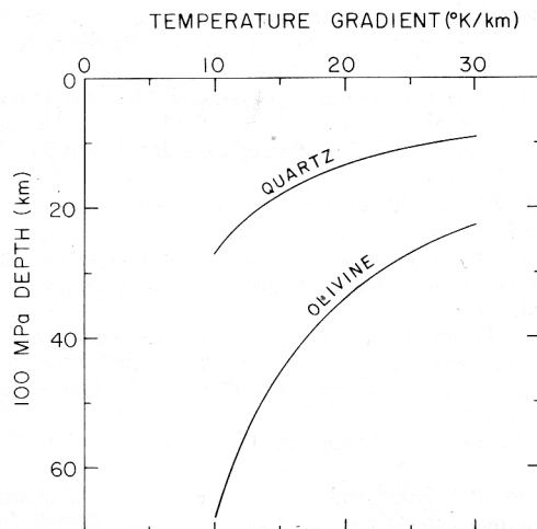
Fig. 6. Depth below which strength is less than 100 MPa as a function of temperature gradient.
