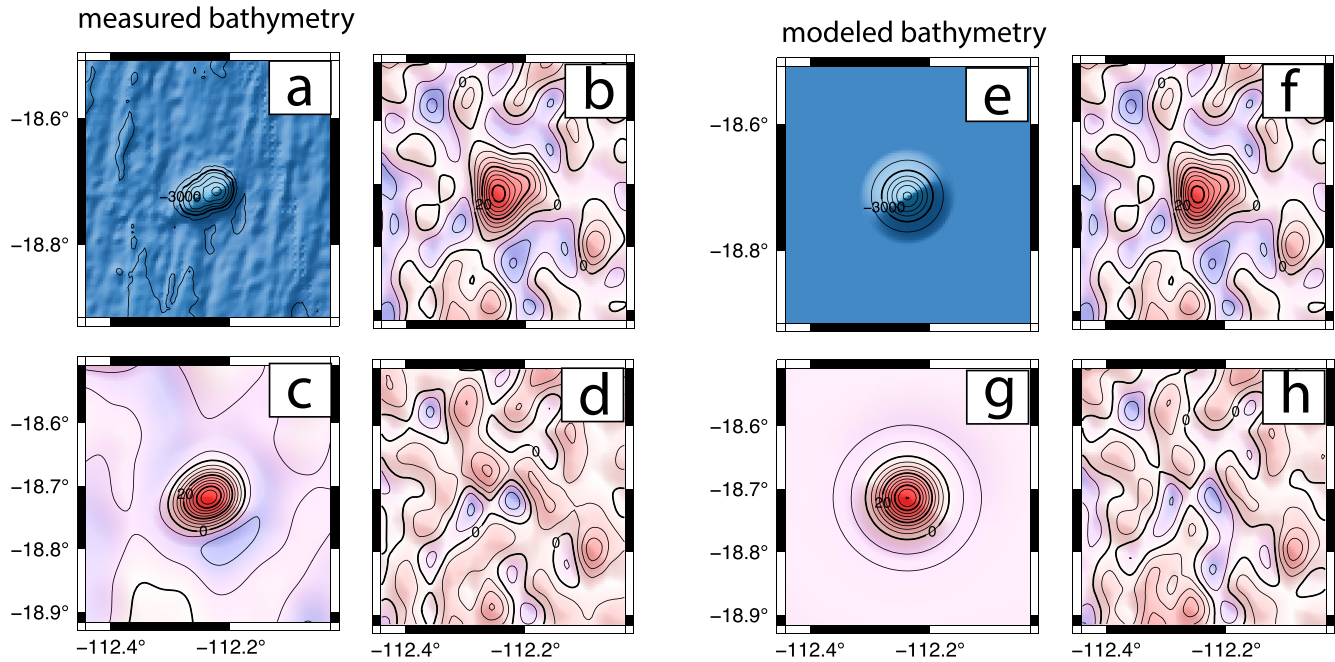
Figure 6. (a) Bathymetry of the smallest of the three seamounts, New-08049 (200 m contours). (b + f) Measured VGG for seamount (5 Etopos contours). (c) Model VGG using a density of 2,800 \text{ kg m}^{-3} . (d) Difference between observed VGG and model VGG (L1 4.54 Etopos, 5 Etopos contours). (e) Model bathymetry using a Gaussian seamount. (g) Model VGG for Gaussian bathymetry (200 m contours). (h) Difference between observed VGG and conical model VGG (L1 5.13 Etopos, 5 Etopos contours).
